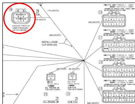
Picture 2. Main Harness
