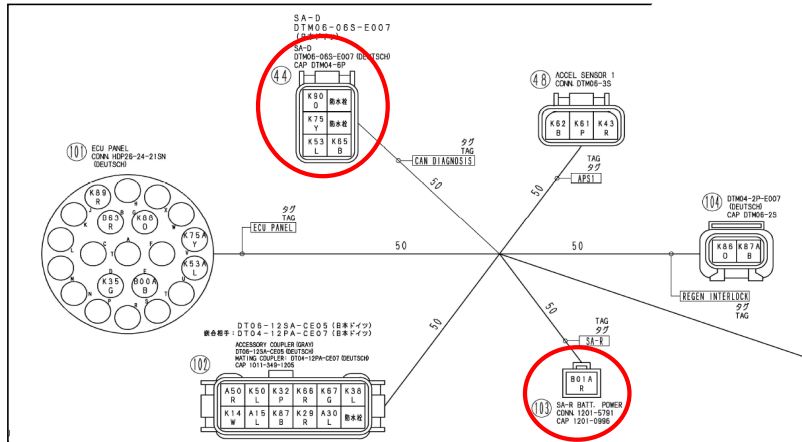
Picture 2. Main Harness
